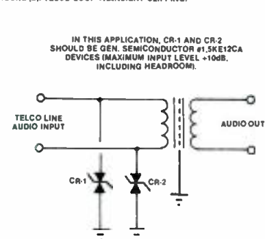
FIGURE (D). TELCO LOOP TRANSIENT CLIPPING.
