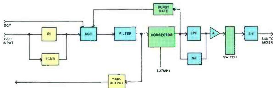
Figure 1. The automatic phase-control circuit maintains the correct phase during both playback and record by tracking the 4.27MHz oscillator with the horizontal sync jitter.
