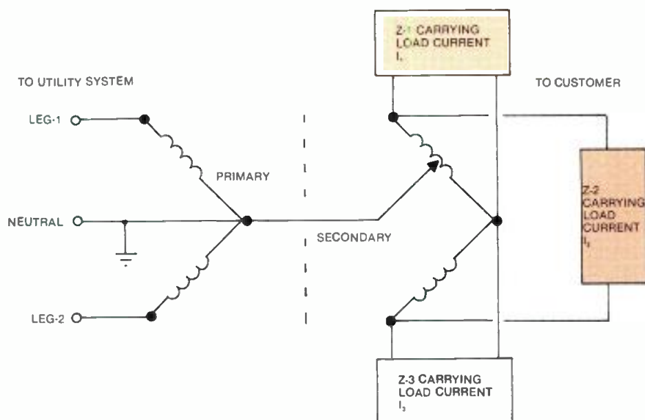
Figure 18. The Open-Delta (or V-V) utility-company service connection. Use of this configuration is not recommended because of the system's poor voltage regulation, high third-harmonic content and transient disturbance propagation characteristics.
